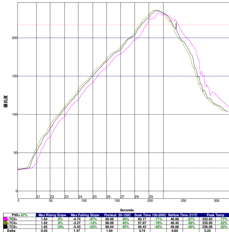
Figure 5 - Example solder reflow profile (AMWx36-E03 evaluation board)
